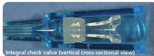
Integral check valve (vertical cross-sectional view)
